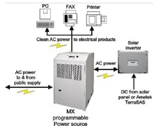
Figure 1. The MX Series power source can deliver power to and receive power from a solar inverter.
