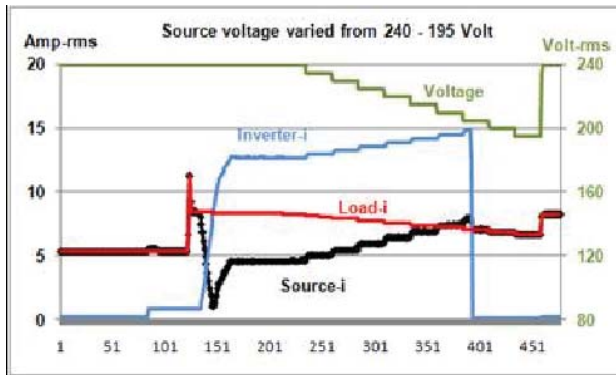
Figure 10: Current flow as the voltage steps in the Transient List are executed
