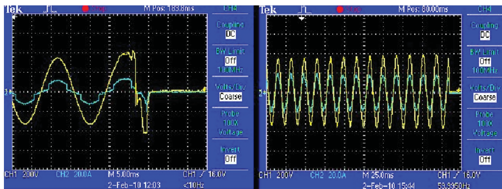
Figure 12: Inverter disconnecting with unbalanced (left) and balanced (right) load
