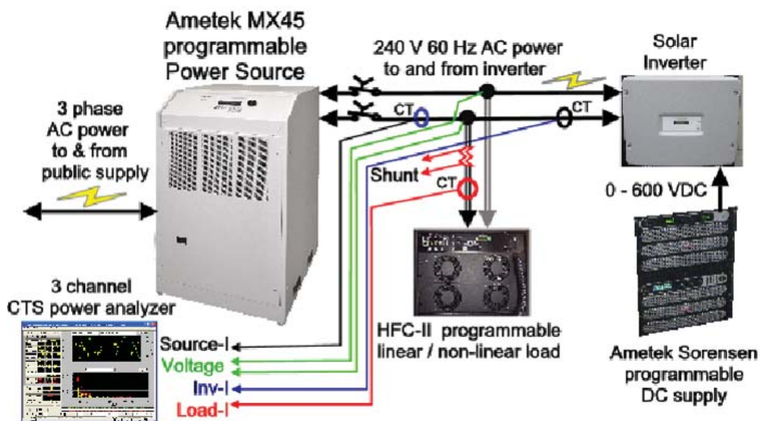
Figure 2: Inverter test setup to illustrate the Regenerative Mode of the Ametek MX Series
